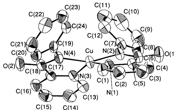
Fig. 1 The molecular structure of [\text{CuL}_2]_2 showing the atom labelling scheme
