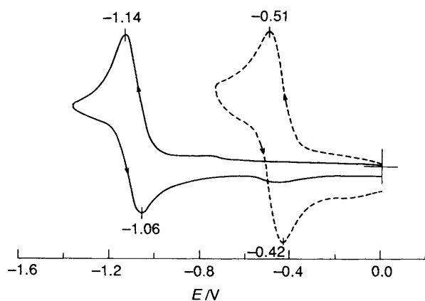
Fig. 3 Cyclic voltammograms of [\text{CuL}^1]\cdot\text{H}_2\text{O} 1 (—) and [\text{CuL}^2] 2 (---) at concentrations of ca. 0.8 \times 10^{-3} \text{ mol dm}^{-3} in dmf (0.15 mol \text{dm}^{-3} \text{NBu}_4\text{ClO}_4 ) at a glassy carbon electrode (scan rate 50 \text{ mV s}^{-1} )
